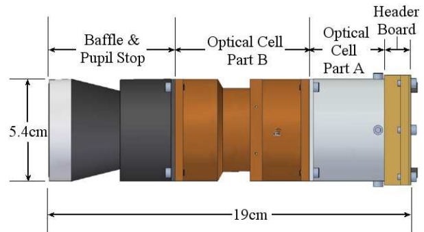
Figure 4: Photometer Housing
