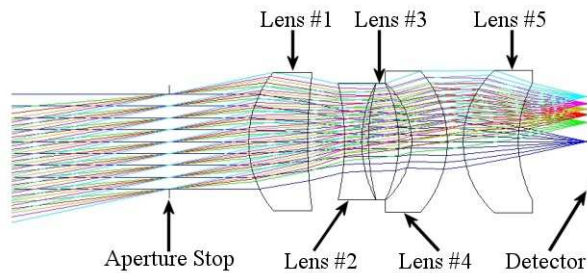
Figure 3: Optics Design
