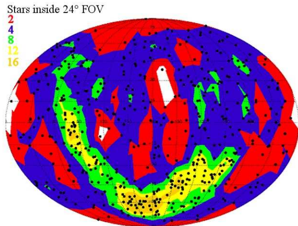
Figure 1: Number of Stars with Limiting Magnitude V=+3.5 Visible Across the Whole Sky for a 24^\circ FOV.
