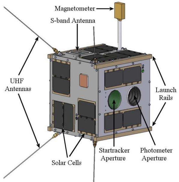
Figure 2: One of Four BRITE Satellites
